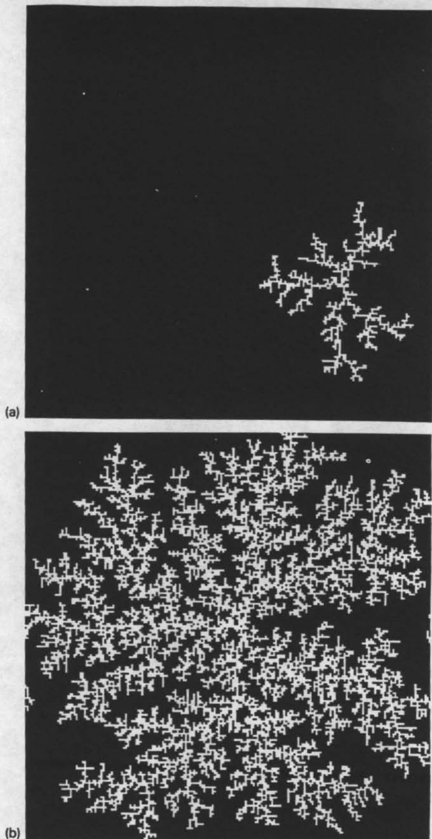
Fig. 2. System size smaller than L_1 . Shown are two stages of the growth for F = 10^{-9} ( L_1 = 500 ) and L = 200 sites. (a) coverage = 0.02, (b) spanning point: coverage = 0.27 (the spanning cluster is light).
