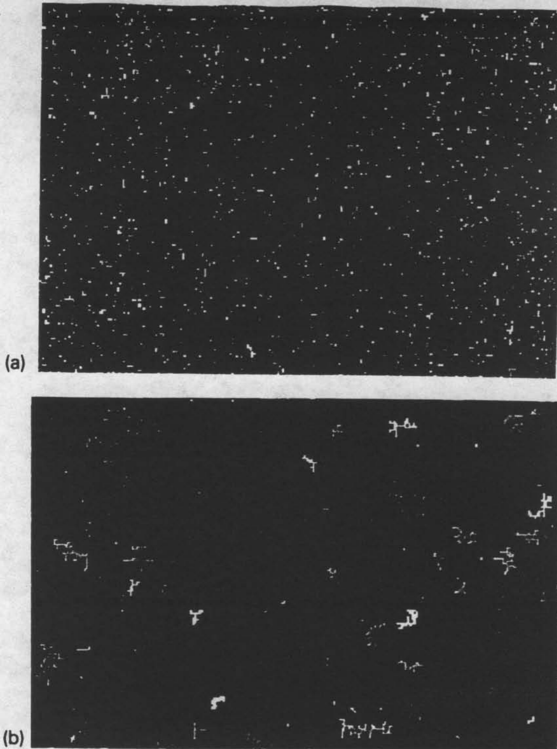
Fig. 1. Influence of diffusion. (a) and (b) are snapshots of two systems at the same fraction of occupied sites or "coverage" (0.15), same size ( L = 400 ) but with different fluxes. (a) F = 10^{-4} (no diffusion), (b) F = 10^{-2} .
